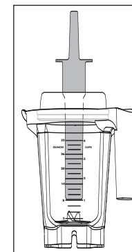
Fig. 3 – Current Accelerator Tool/Tamper in Container
