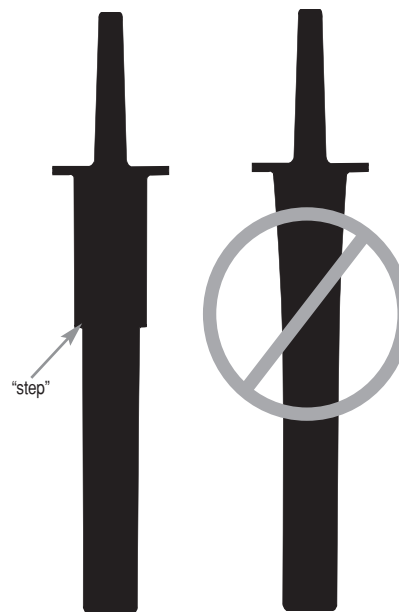
Fig. 1 – Current Accelerator Tool/Tamper
